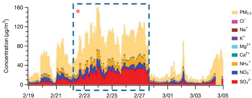
Fig. 6. Timelines of PM 2.5 , Cl - , Na + , K + , Mg 2+ , Ca 2+ , NH 4 + , NO 3 - and SO 4 2- from February 19 th to March 05 th , 2014.
